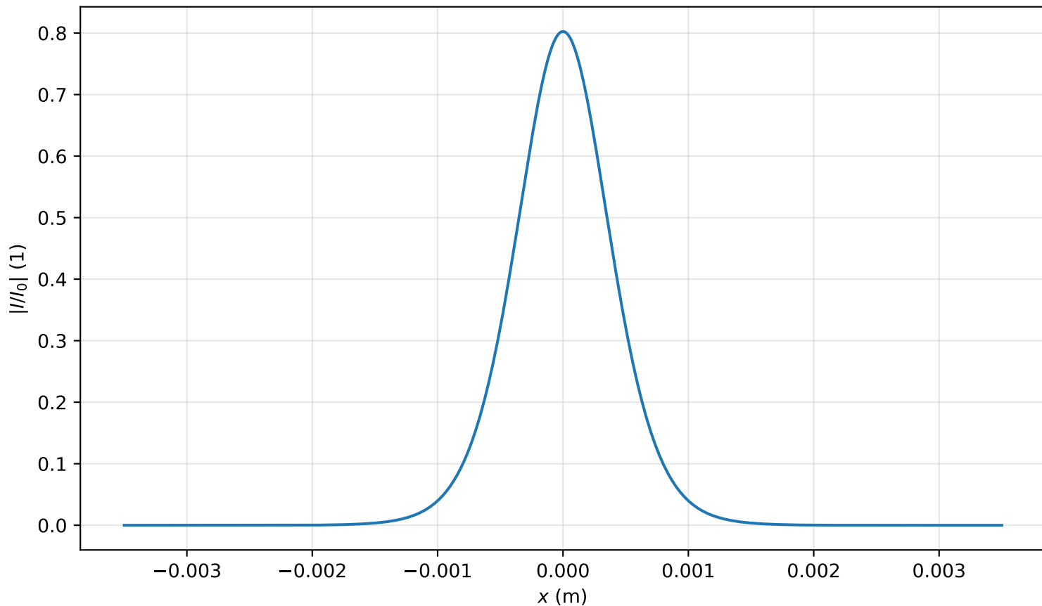
Intensity profile I(x, y = 0, z = 2.070m)/I_0 , P_{in}=0.5P_{cr} , artificial time
